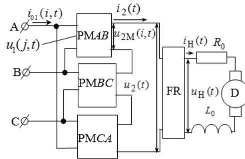
Figure 1. Schematic diagram of the converter
